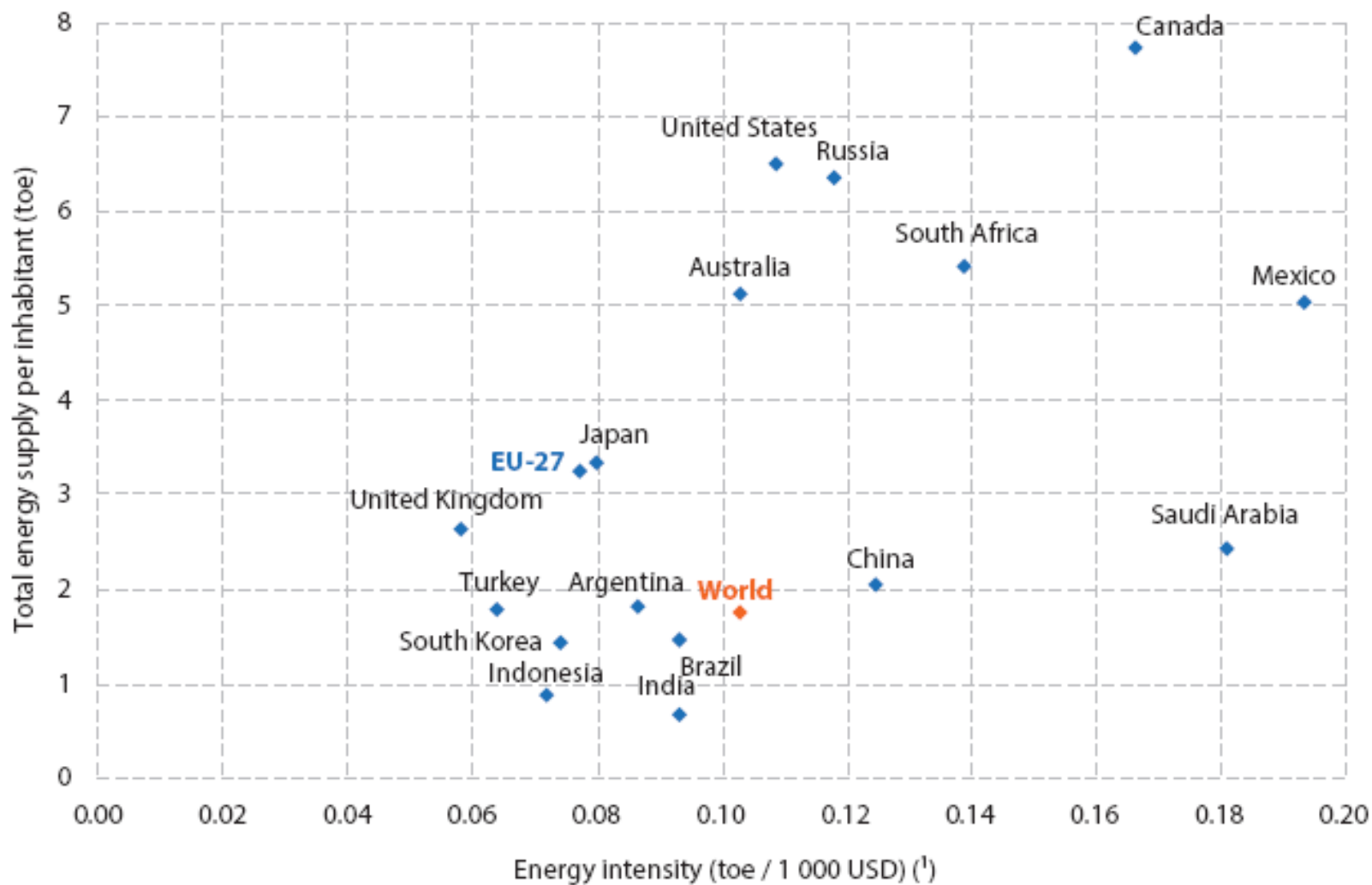
Figure 12.7: Energy intensity, 2017
